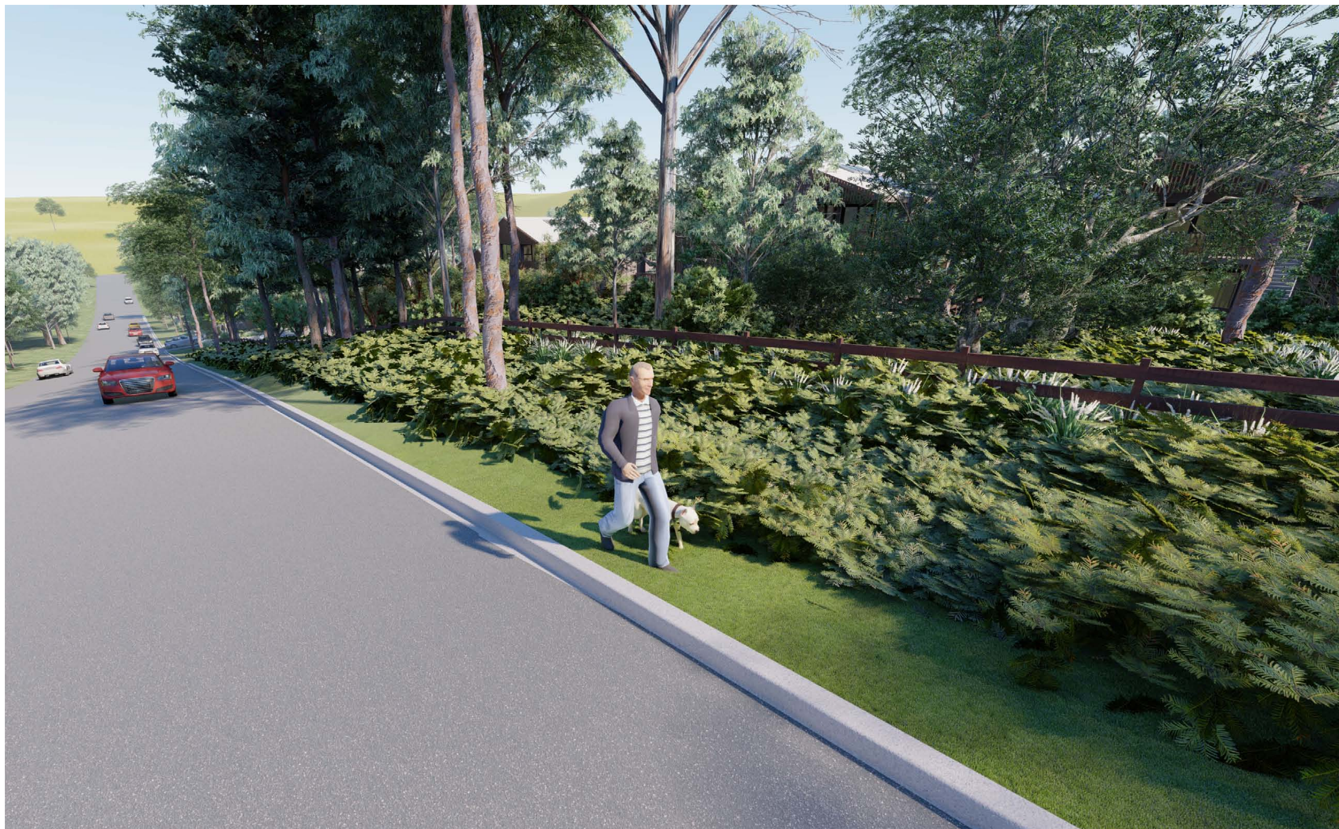
Detailed eye-level view along Cooyong Road frontage illustrating kerb and gutter and grassed footway
